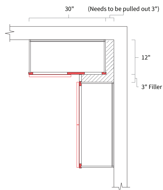
Installation Diagram
