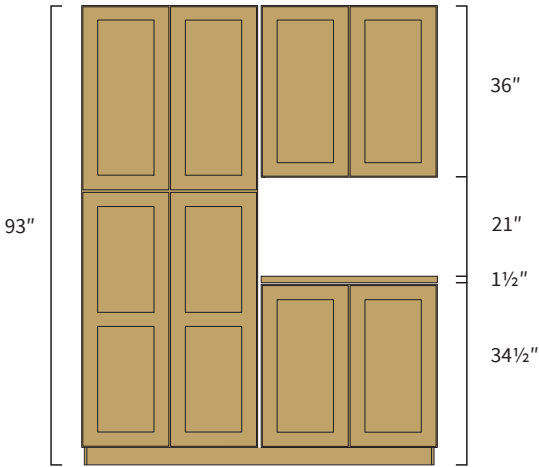
8' Ceiling With 36" Tall Wall Cabinet
