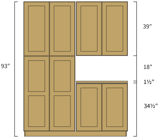
8' Ceiling With 39" Tall Wall Cabinet
