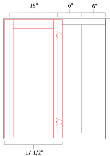
Opening Dimensions
